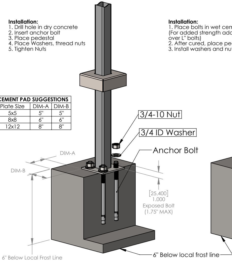
STUD-ANCHOR-KIT Installation Best for existing concrete
