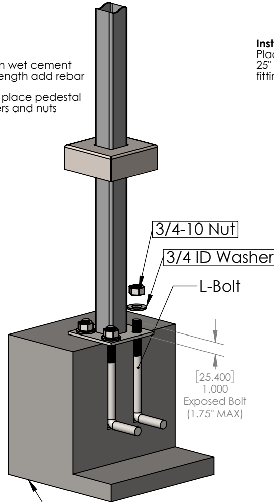
L-BOLT-KIT Installation Best for new cement
